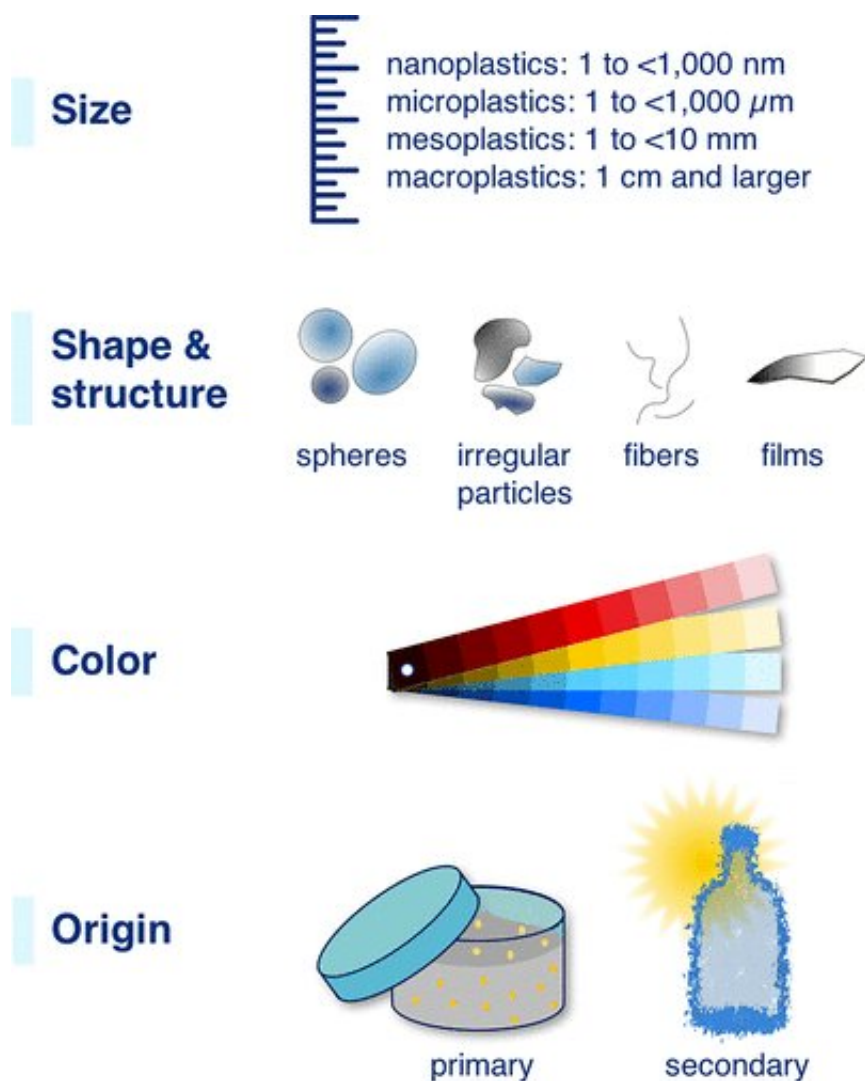
Figure 1. Major characteristics of nano- and microplastic particles. Figure and definitions of size categories (nanoplastics: 1 to
