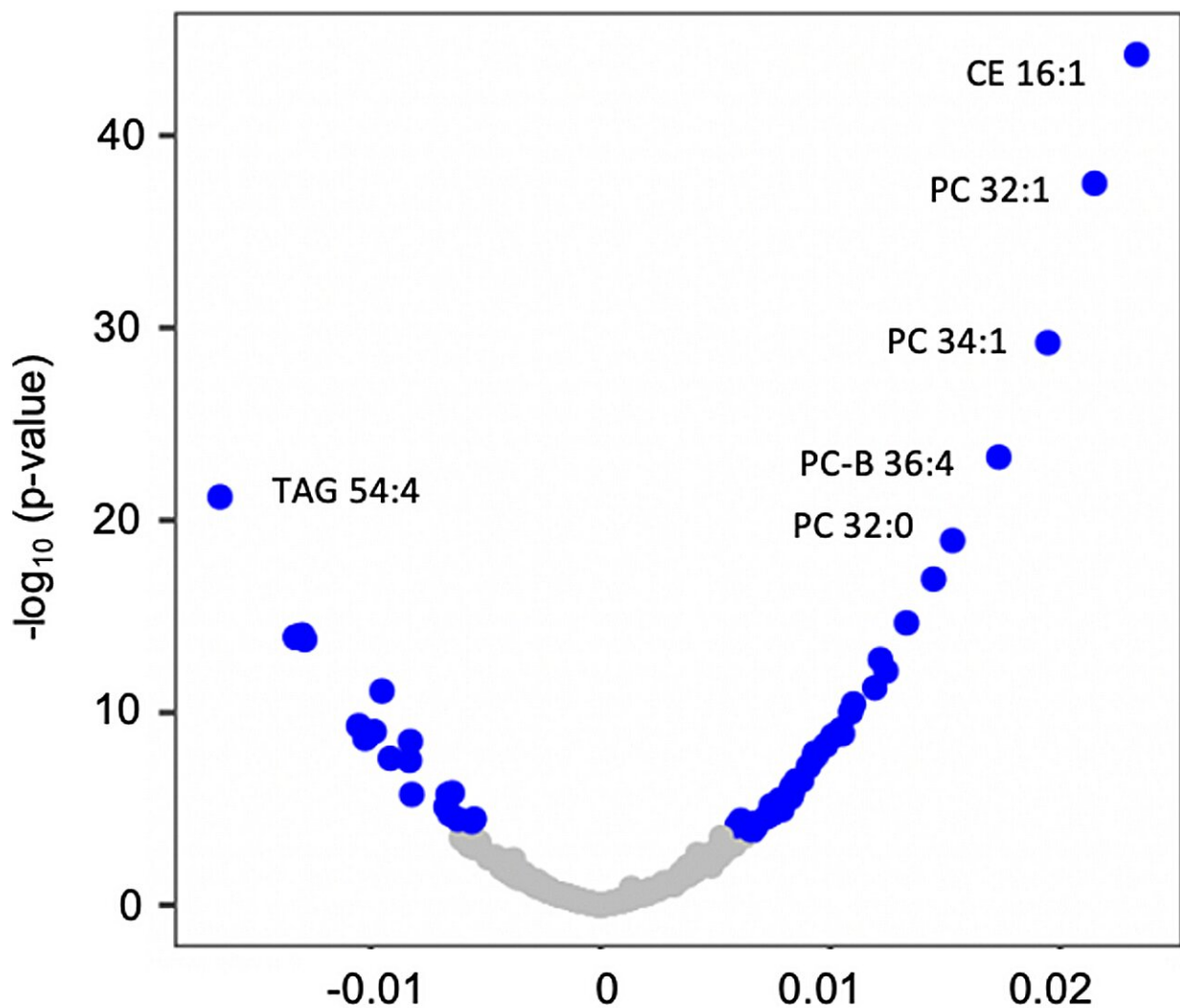
Change in the level of metabolites in response to 1 gram/day alcohol consumption
