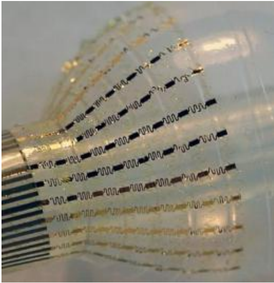
Fully inflated multifunctional balloon instrumented with temperature, tactile and EKG sensors on islands interconnected by non-coplanar serpentine wires. Credit: Dae-Hyeong Kim, University of Illinois
