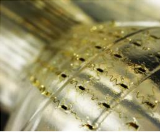
Fully inflated multifunctional balloon instrumented with temperature, tactile and EKG sensors on islands interconnected by non-coplanar serpentine wires. Credit: Darren Stevenson, University of Illinois
