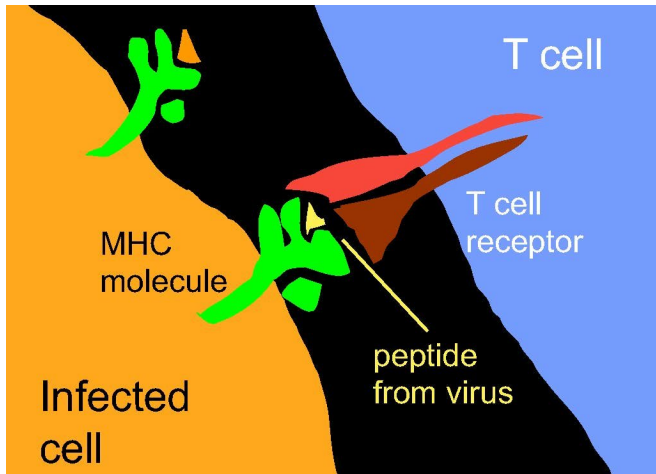
Killer T cells detect a broad range of viral targets. Credit: A. Moosmann/Helmholtz Centre Munich
