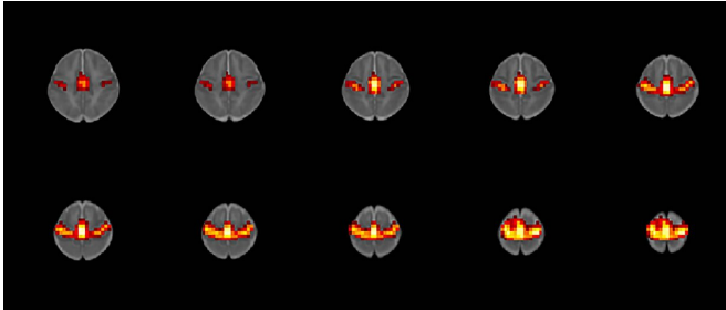
Group independent component analysis of resting state functional MRI obtained as a part of this study showing one of the resting state networks of the brain. Credit: Study author and RSNA
