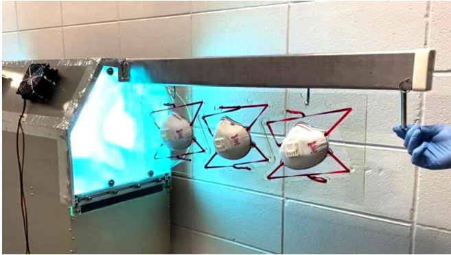
A prototype of the self-contained disinfection unit. Credit: Peter Eng
