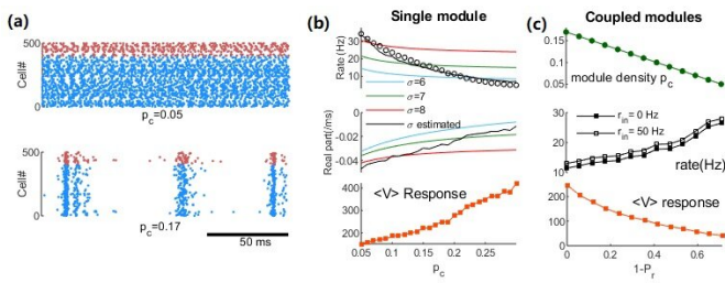
(a) Examples of the neuron firing patterns in modules of different densities; (b) The dynamic properties of a single separate module change with its connection density, predicted by the mean-field theory; (c) The mean-field theory predicts the dynamic transition during the rewiring process of the whole network. Credit: Science China Press
